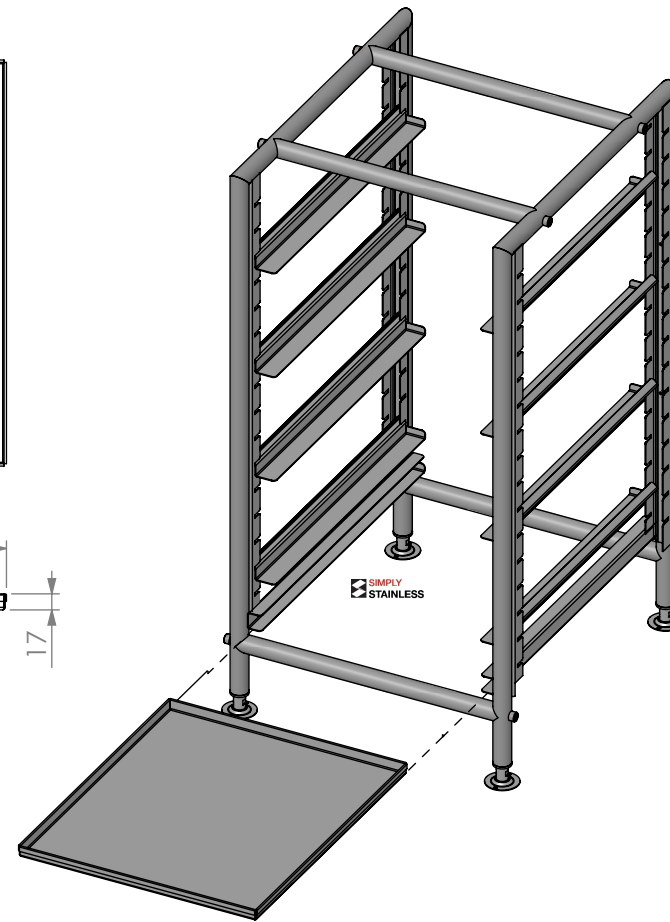
Drip Tray
