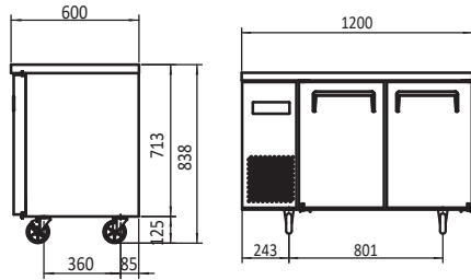
YPF9020/YPF9025 side view
