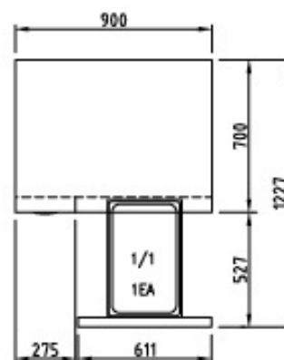
PLAN VIEW
