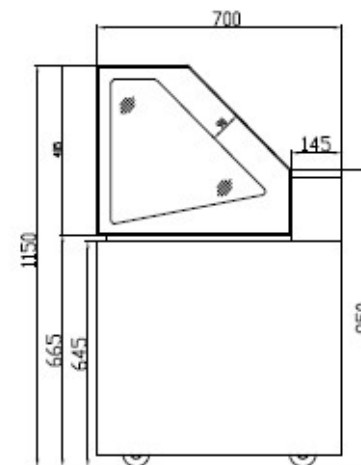
SIDE VIEW 左侧视图
